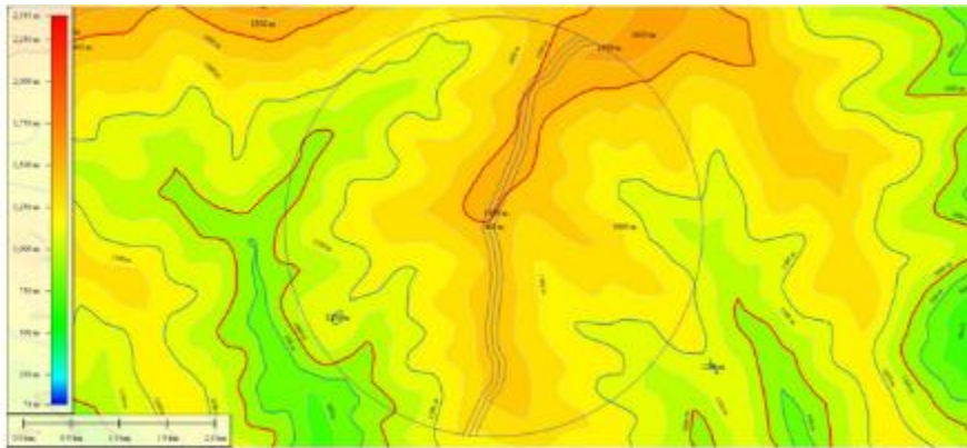
Fig. 15 - Generate Area Features Colored Based on the Current Elevation Shader in Addition to Contours, E=100 m
