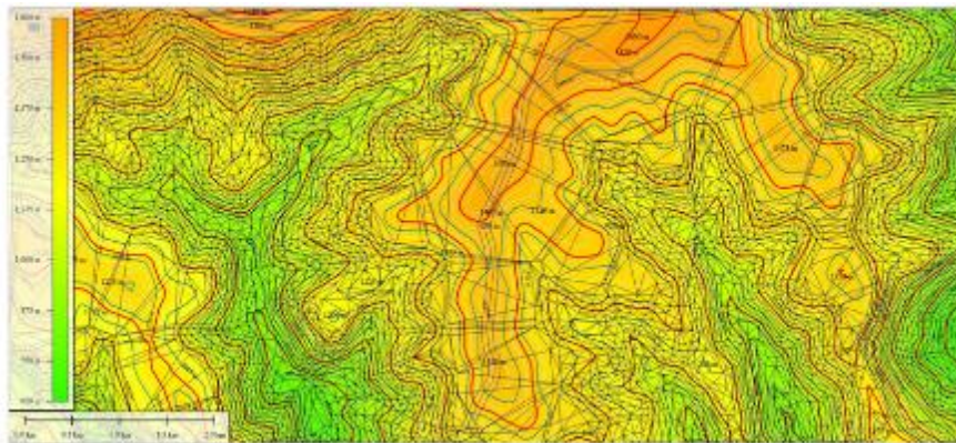
Fig. 16 - Create elevation Grid from 3D Vector Data - Triangulation Network (TIN)
