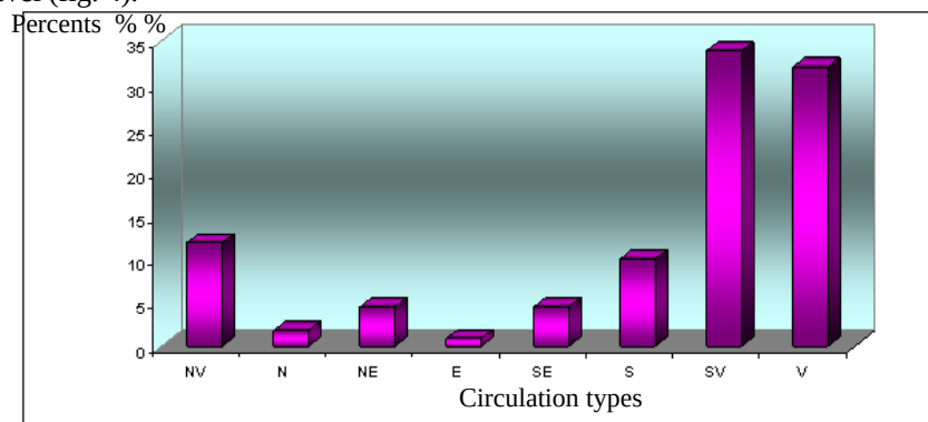
Fig. 3. Atmospheric circulation types for torrential rains.
