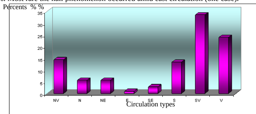
Fig. 5. Atmospheric circulation types for hail.
