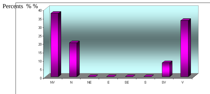
Fig. 7. Atmospheric circulation types for hoarfrost.
