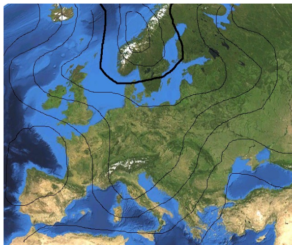
Fig. 2. Typical geopotential field configuration (500 mb) for squalls situations
