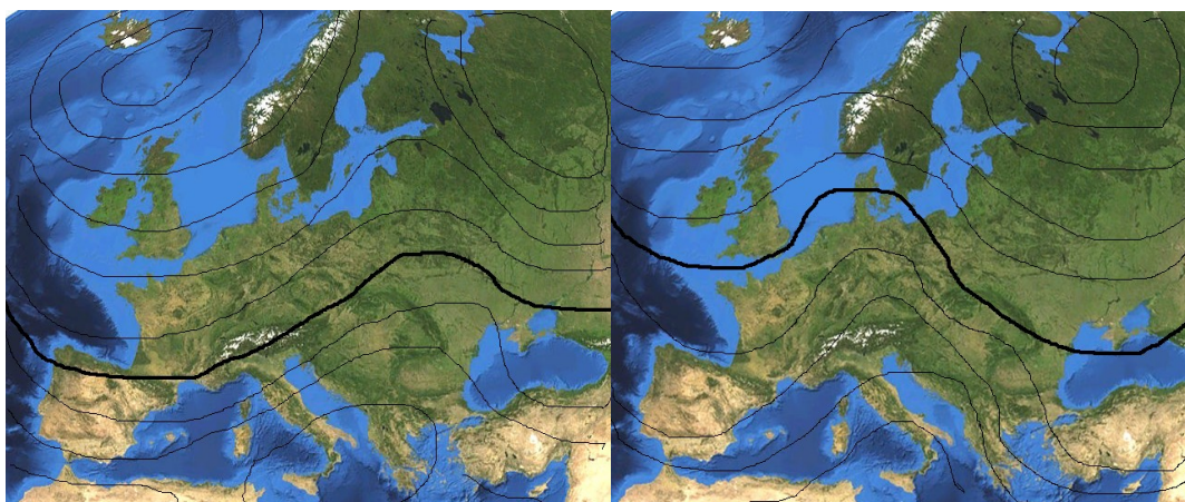
Fig. 10. Typical geopotential field configuration (500 mb) for gaze ice situations.
