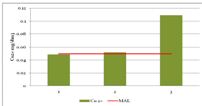
Fig.3. Copper content of shallow groundwaters from Sag
