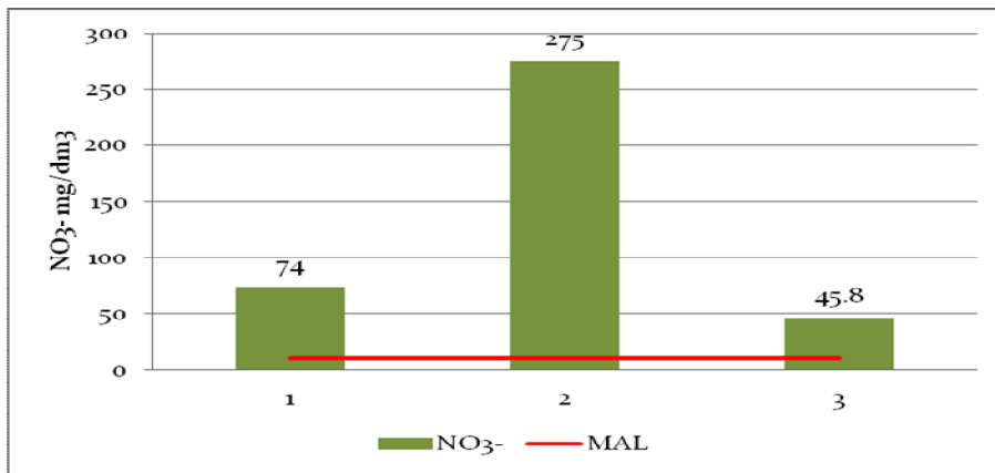
Fig.1.Nitrate content of shallow groundwaters from Sag
