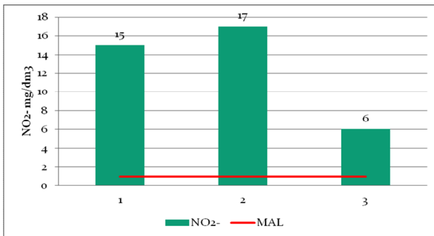
Fig.2.Nitrite content of shallow groundwaters from Sag
